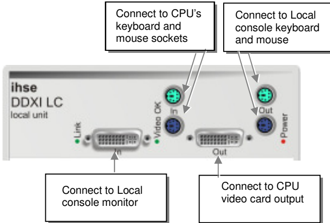
Figure 3 K436-1W Local Unit
