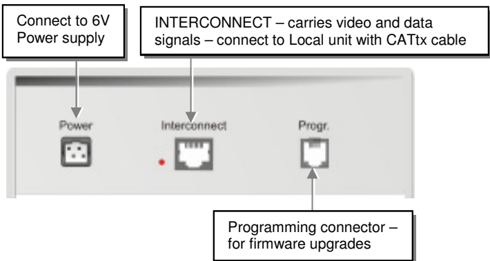
Figure 4 K436-1W Local/Remote Unit
