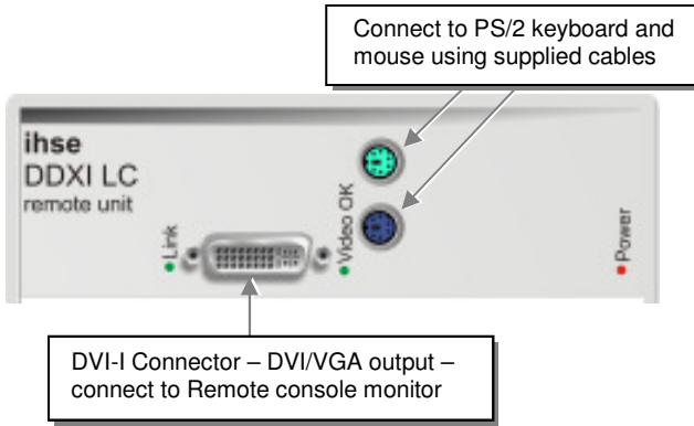
Figure 2 K436-1W Remote Unit
