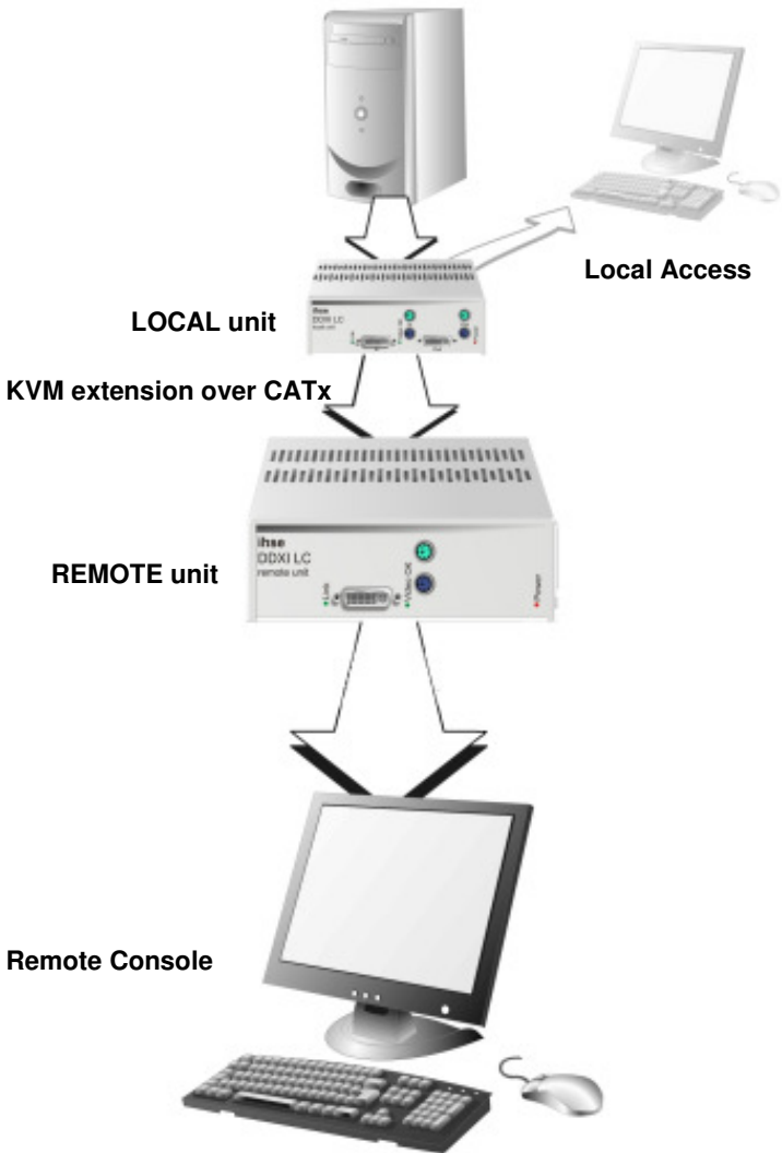
DDXI/LC KVM extender system
