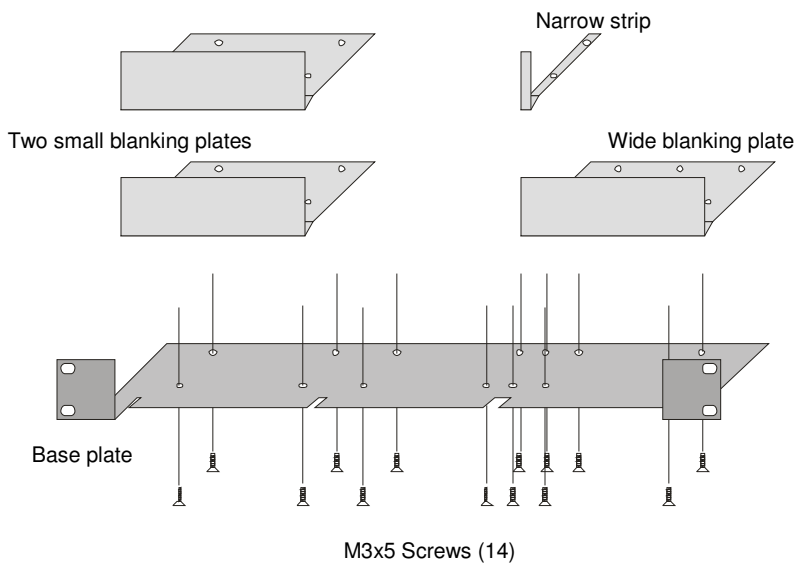
Figure 19 Rack Mounting Kit
