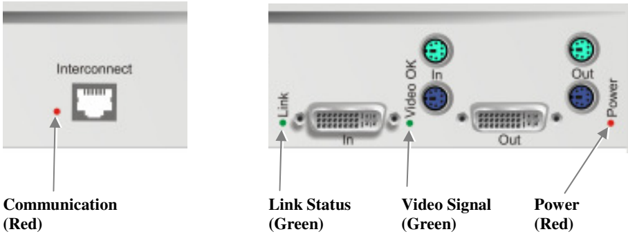
Figure 5 K436-1W Local/Remote Unit
