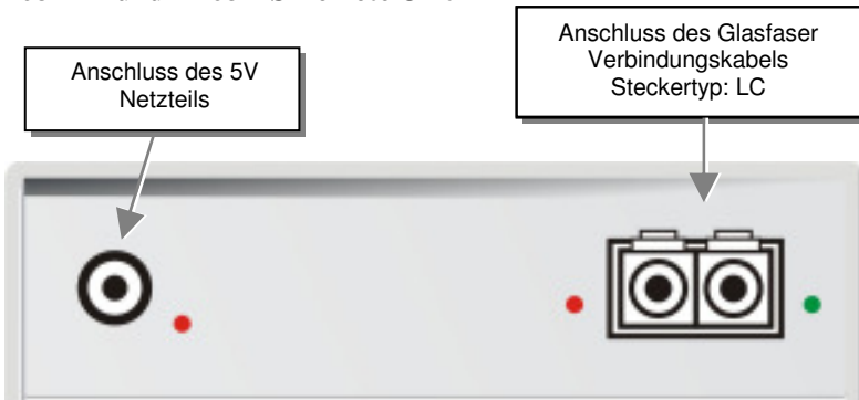
DVXi/ME Media-Extender Typ K466-0M, K466-AM, K466-0S, K466-ASW, K467-0M, K467-AM, K467-0S, K467-AS, K468-0M, K468-AM, K468-0S und K468-AS Local Unit und Remote Unit
