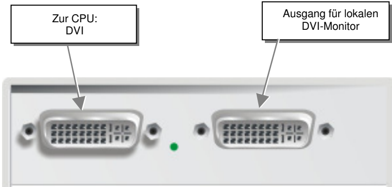
DVXi/ME Media-Extender Typ K466-0M, K466-0S, K467-0M, K467-0S, 468-0M und K468-0S Local Unit
