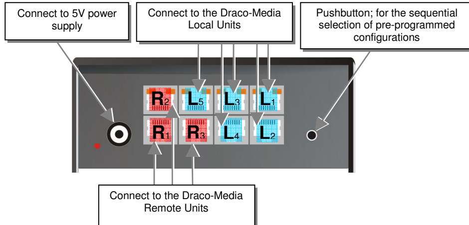
Draco-minor Switch – as Crosspoint-Switch 5x3
