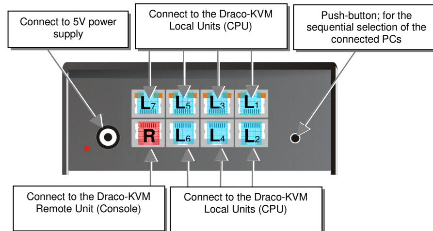
Draco-minor Switch – as Single-Head KVM-Switch
