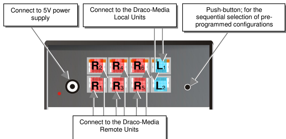
Draco-minor Switch – as Crosspoint-Switch 2x6
