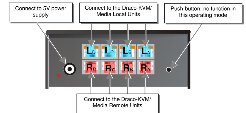
Draco-minor Switch – as 4x 1to4 Multiplex- Repeater
