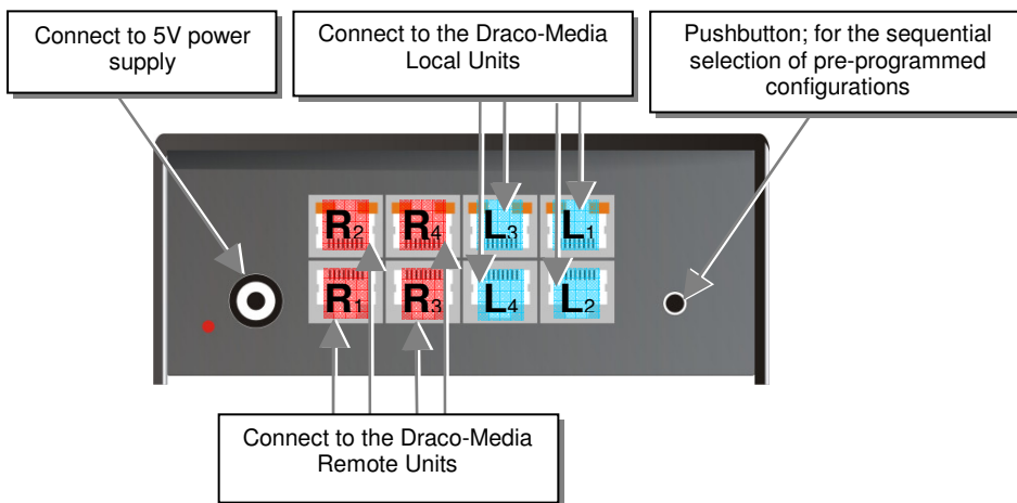
Draco-minor Switch – as Crosspoint-Switch 4x4
