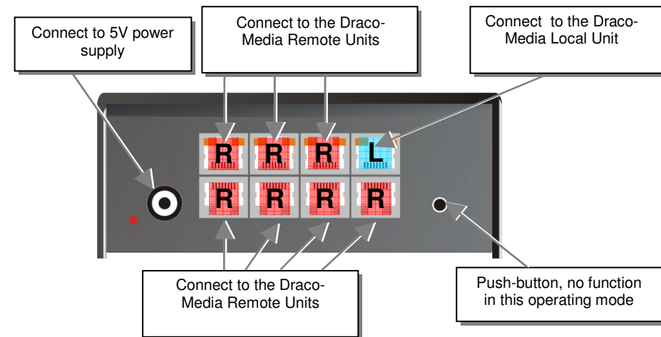
Draco-minor Switch – as 1to7 Multiplex-Repeater
