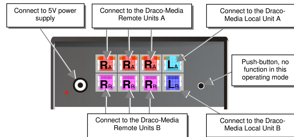
Draco-minor Switch – as 2x(2to3) Multiplex-Repeater
