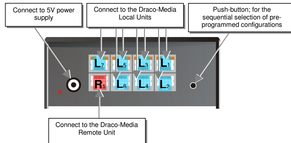
Draco-minor Switch – as Crosspoint-Switch 1x7
