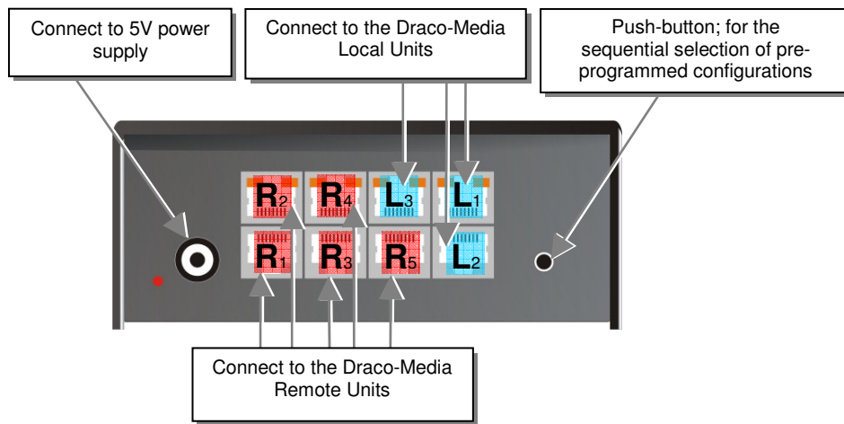
Draco-minor Switch – as Crosspoint-Switch 3x5
