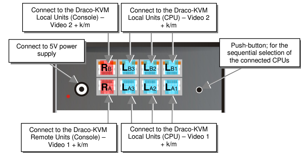
Draco-minor Switch – as Dual-Head KVM-Switch
