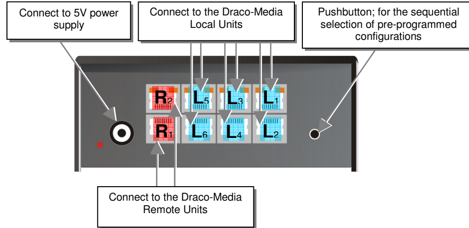
Draco-minor Switch – as Crosspoint-Switch 6x2
